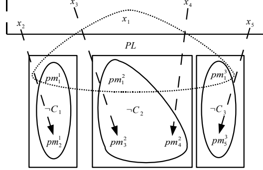
Figure 1: Implementation of pure value rule for one variable x_i
