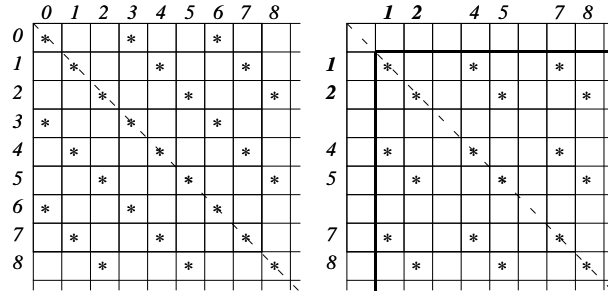
Figure 3: The \lambda -multiples of 3, M_3 , and the square \Sigma_{1,3,\{0,1\}}
