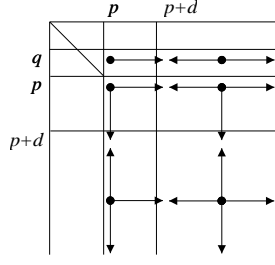
Figure 4: Moving using c^p b^{p+d} and c^{p+d} b^p
