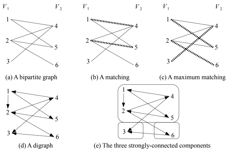
FIGURE 2.1. Examples of graphs
