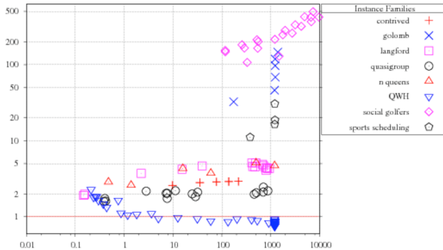
FIGURE 6.1. Speedup of PriorityQ over Simple. The graph is a scatter-plot, with each point comparing results on a single instance. The x -axis represents the run time of Simple to solve the instance. The y -axis gives the speedup obtained by using PriorityQ instead of Simple. A ratio of 1 indicates that the two methods run at the same speed, with ratios higher than 1 indicating that PriorityQ is faster, and ratios less than 1 indicating that Simple is faster. The ratio is calculated by dividing the number of search nodes explored per second by PriorityQ by that for Simple. In this graph we can see that performance ranges from a slight slowdown from using PriorityQ, on some QWH instances, to speedups of hundreds of times on some social golfers instances.
