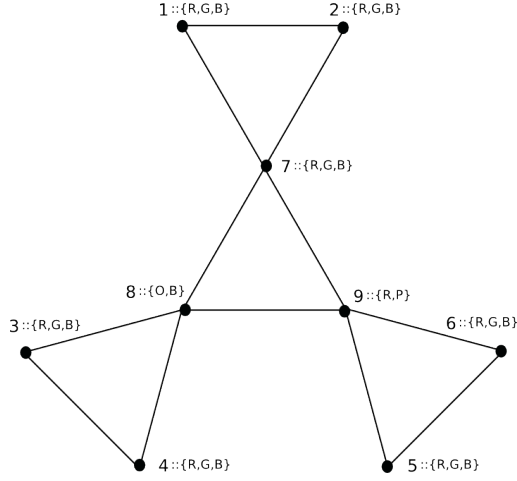
Fig. 2. Example n = 3
